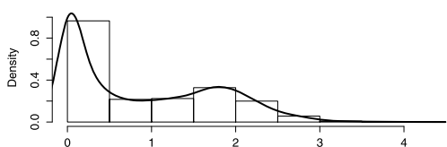
Estimated beta
