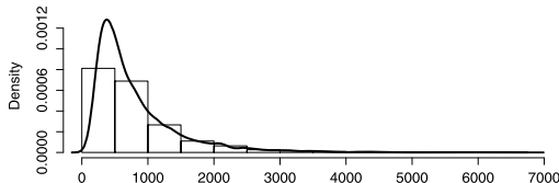
Estimated gamma
